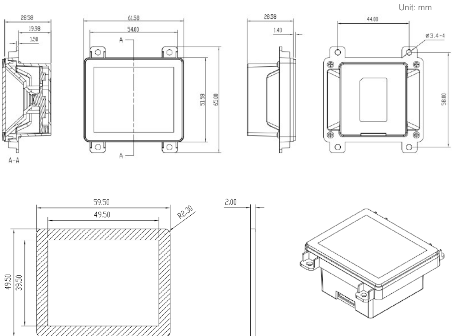
The front cover dimensions
